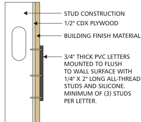
MOUNTING DETAIL SCALE 1"=1'-0"
